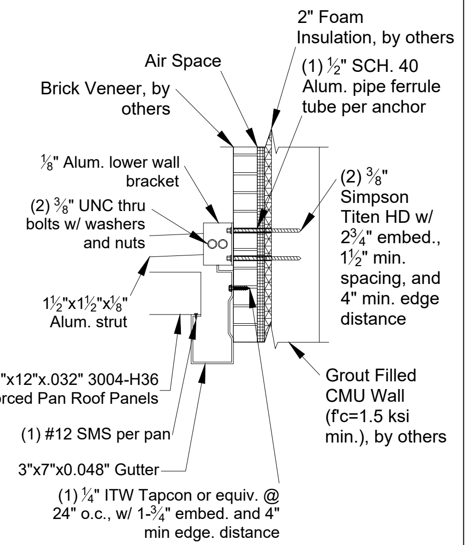
3/11 Rear Gutter Detail
