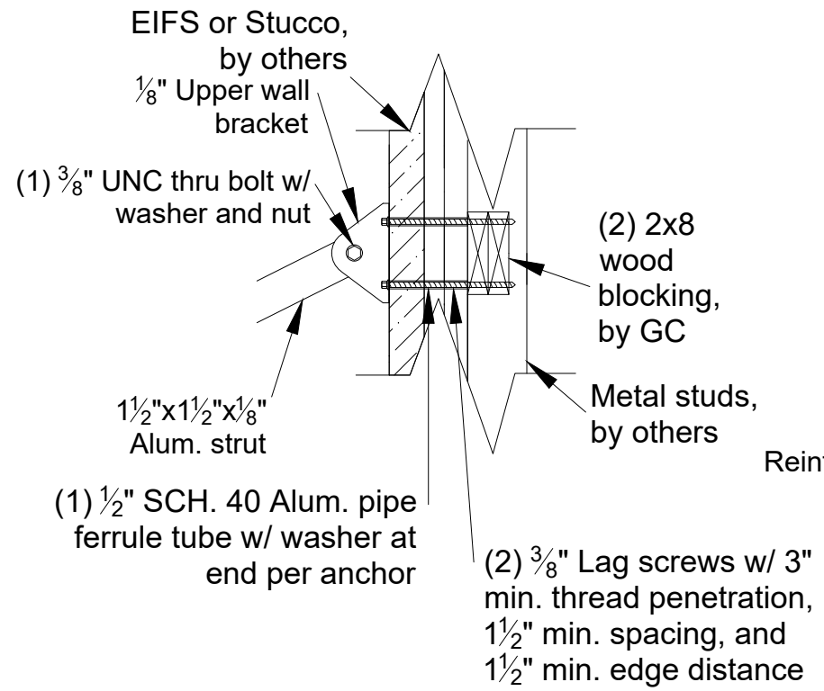
2/13 Wall Bracket Detail
