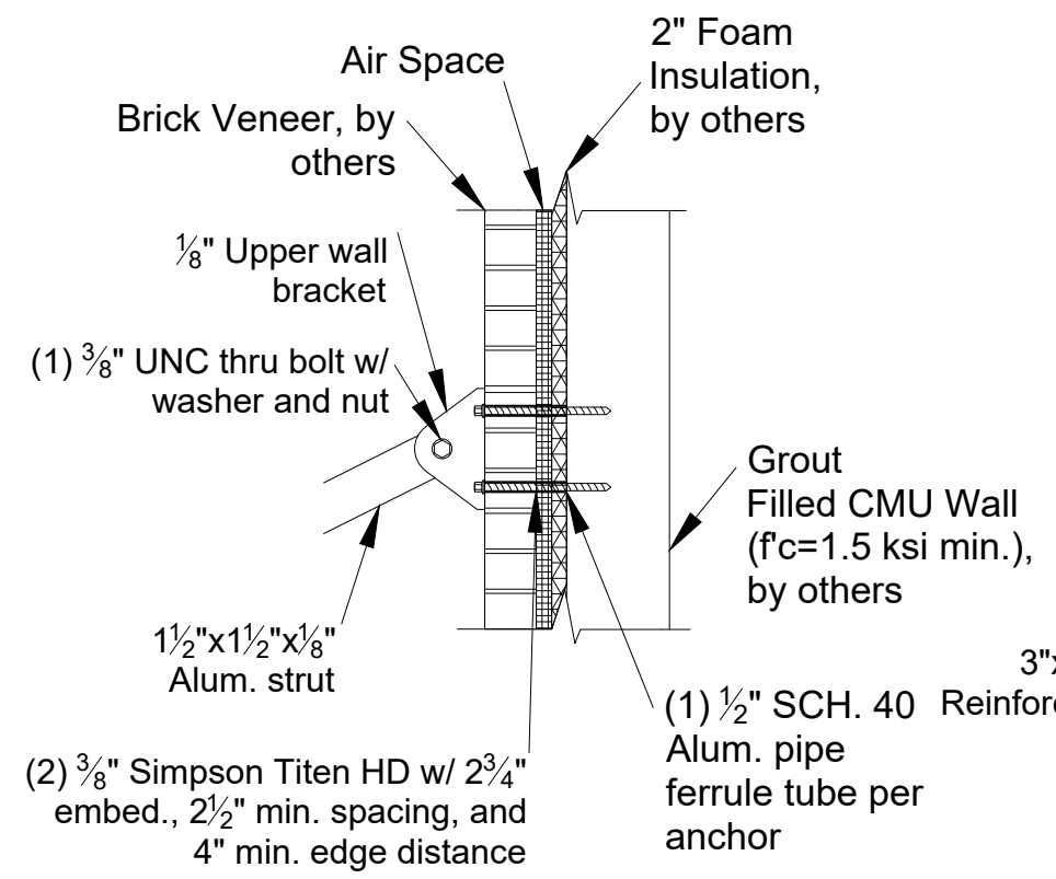
2/11 Wall Bracket Detail
