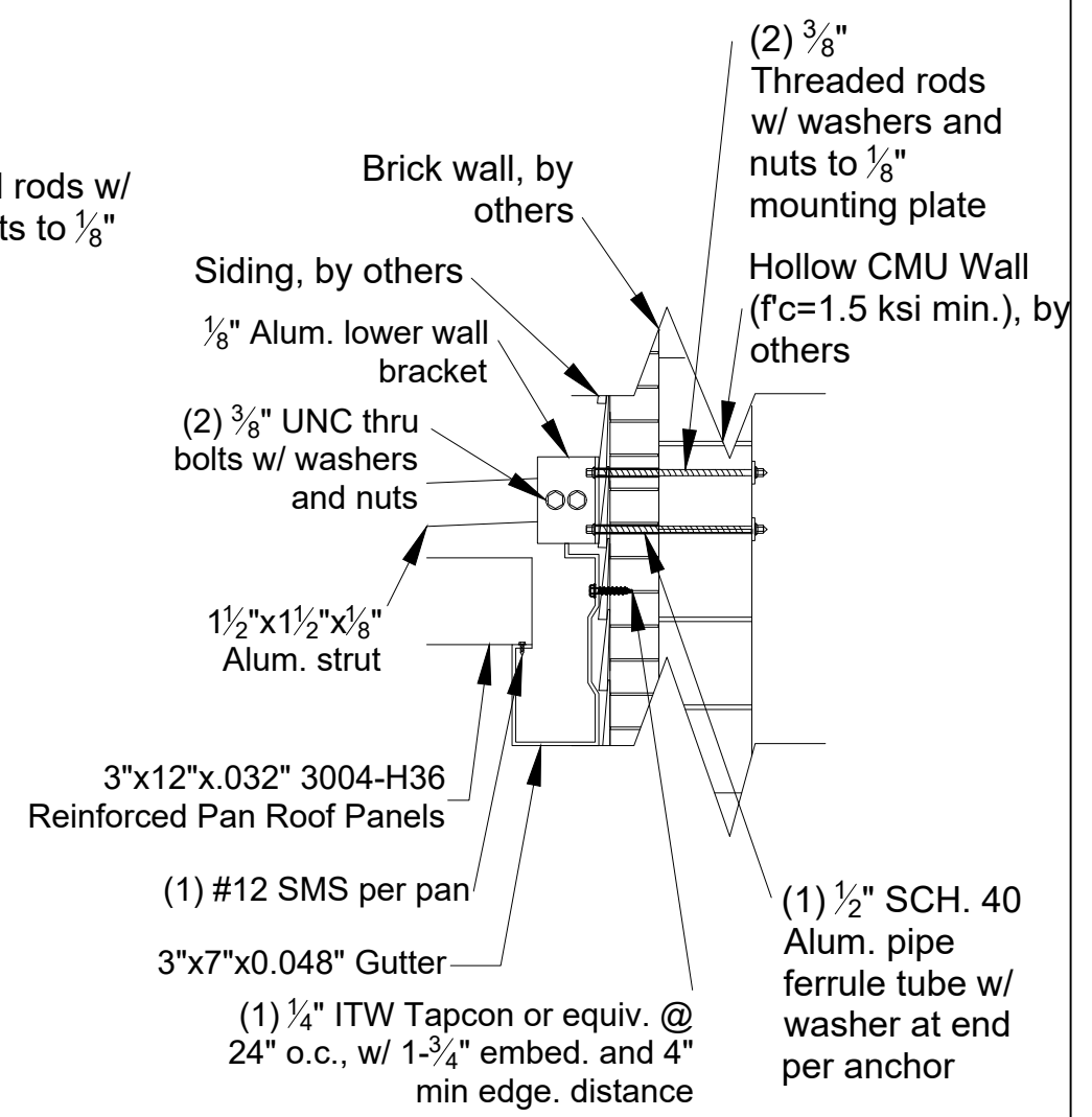
3/12 Rear Gutter Detail
