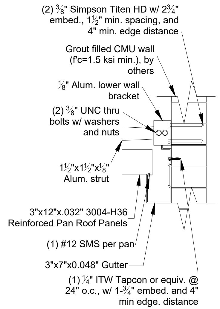
3/10 Rear Gutter Detail
