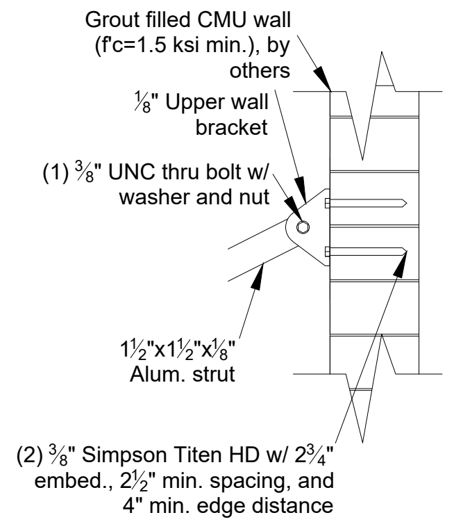
2/10 Wall Bracket Detail
