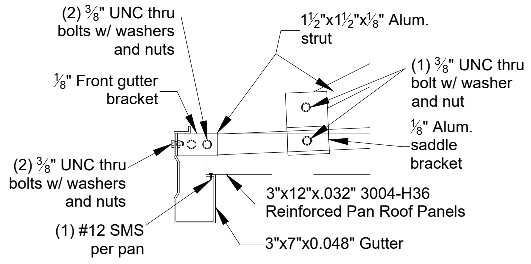
1/11 Front Gutter Detail
