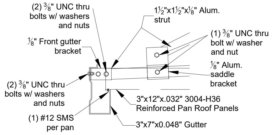
1/13 Front Gutter Detail
