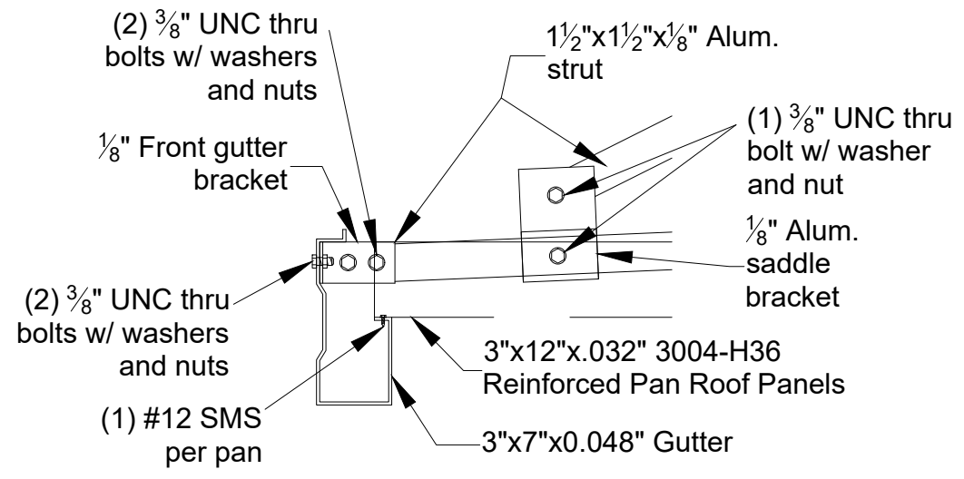
1/9 Front Gutter Detail
