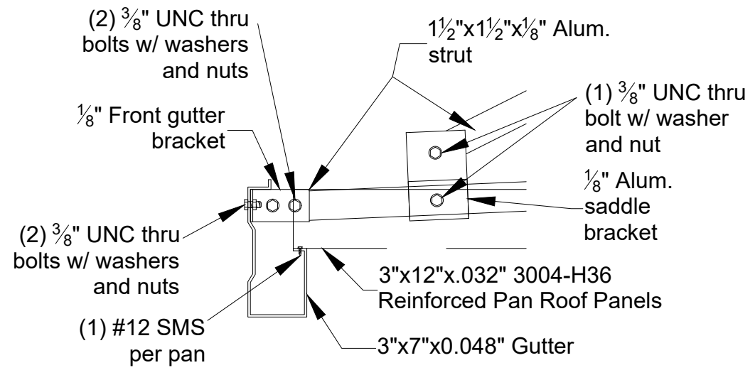
1/12 Front Gutter Detail
