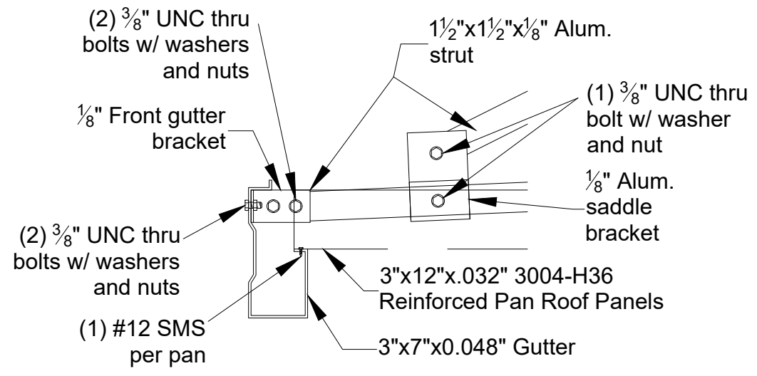
1/10 Front Gutter Detail
