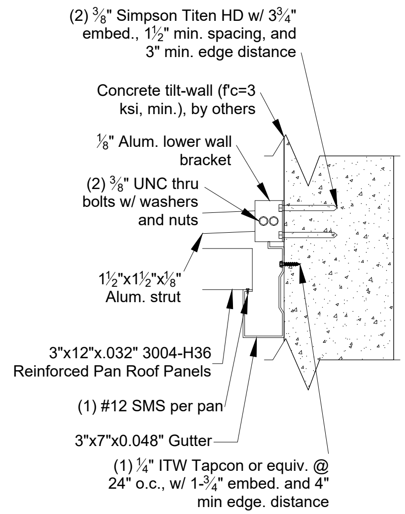
3/9 Rear Gutter Detail
